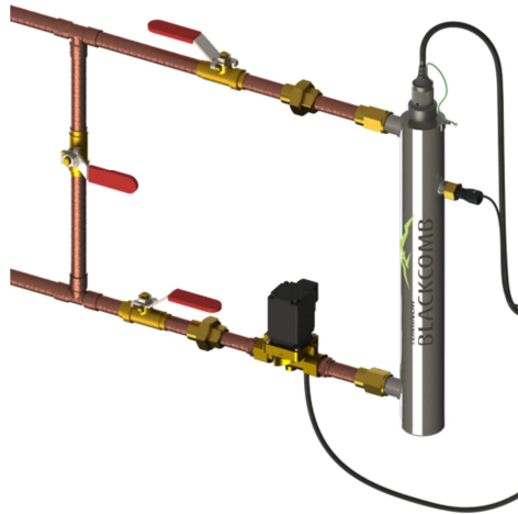
Figure 3. Recommended Installation
