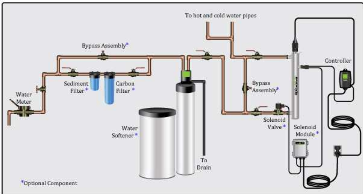
Figure 2. Recommended POE Installation
